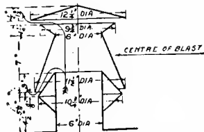
Fig. 4309. THE ROE. TYPES OF VENTILATORS.
